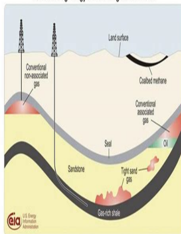
Schematic geology of natural gas resources
